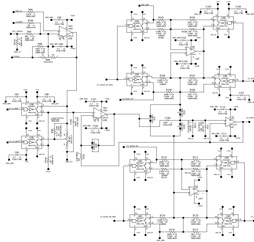
CV RANGE AND SLEW CIRCUITS
