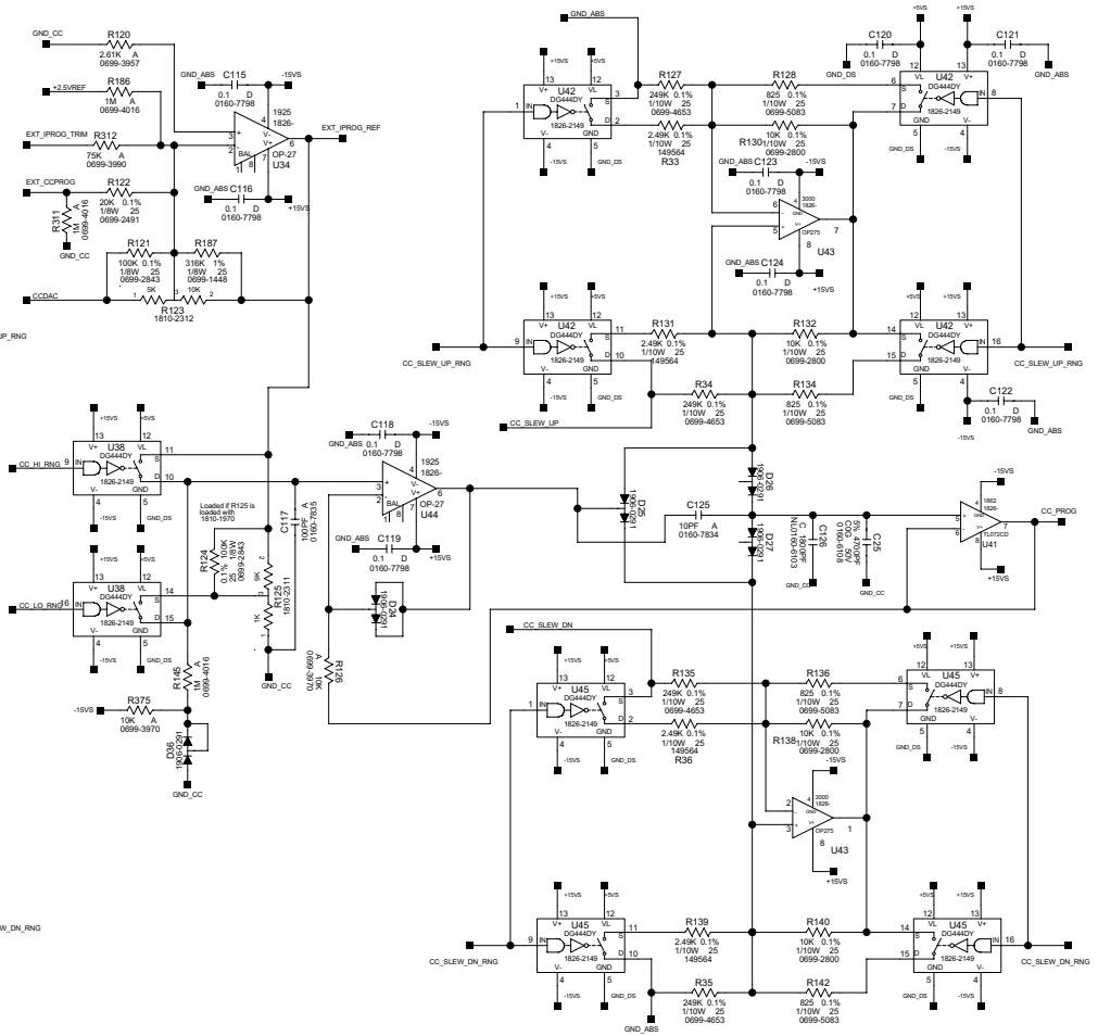
CC RANGE AND SLEW CIRCUITS
